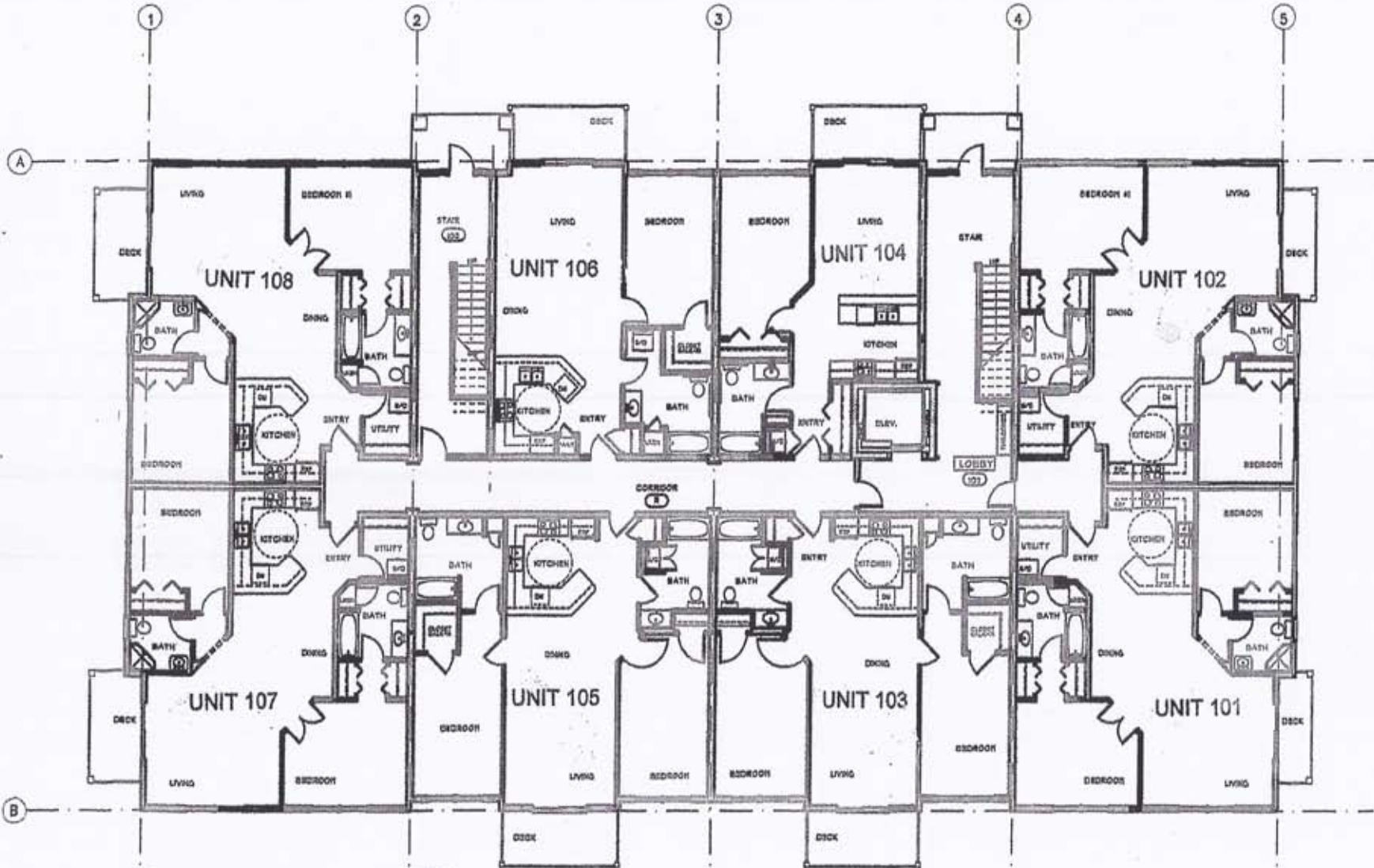
1 FIRST FLOOR PLAN 3/16" = 1'-0"
